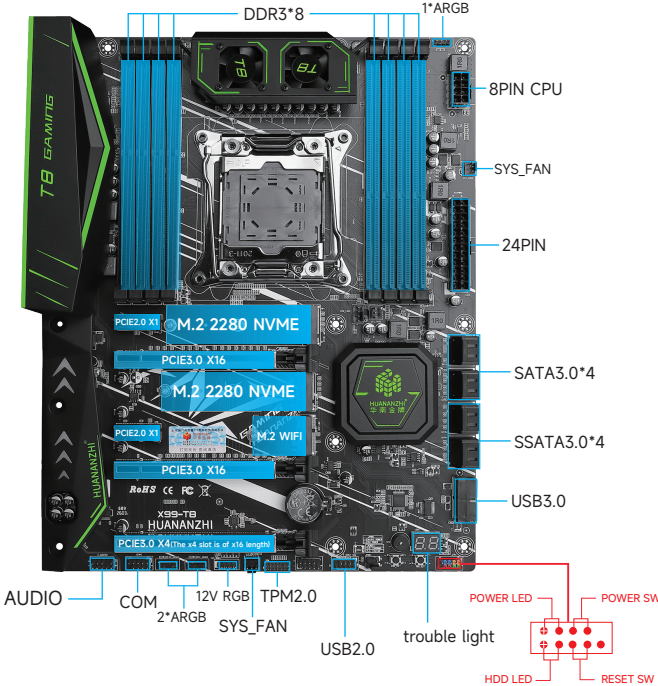
1-1 X99-T8 Motherboard Illustration
