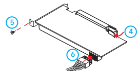
2-9 显卡安装
